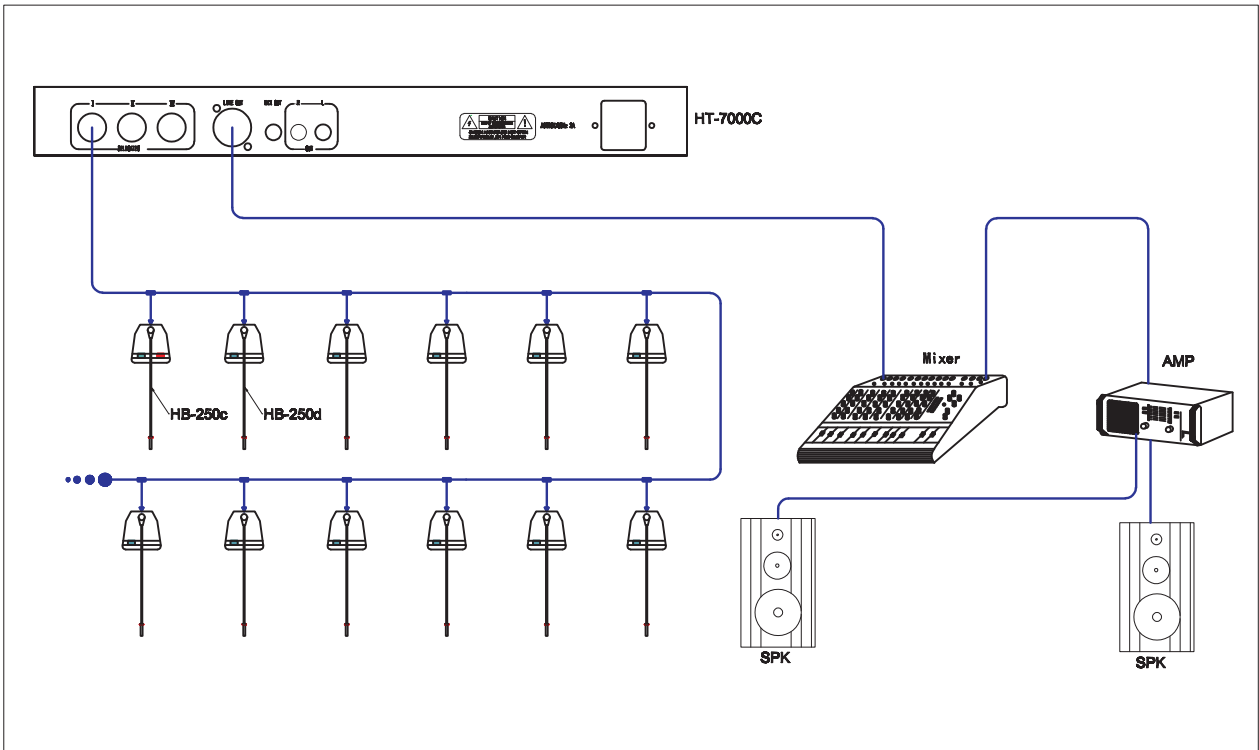
HT-7000C System Connection Diagram
